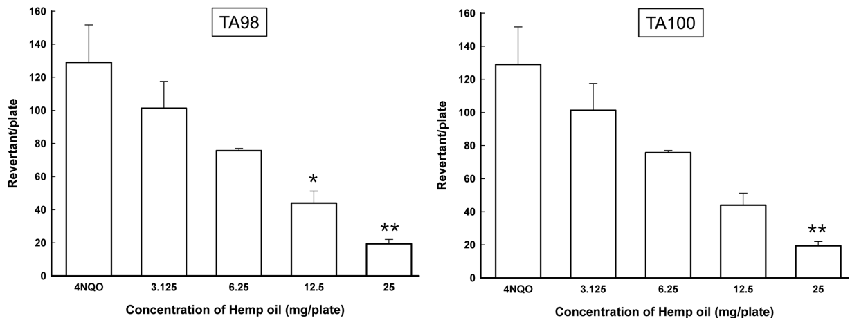
Fig. 2. Antimutagenic effect of hemp seed oil against 4-nitroquinoline 1-oxide (4NQO). The 4NQO was included 0.15 g per plate. * p < 0.05 , ** p < 0.01 .
